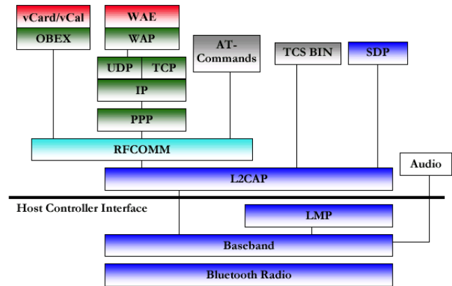
Figure 3. Bluetooth Protocols Stack [13].
